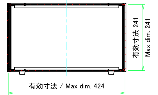
C-C (1:7)
